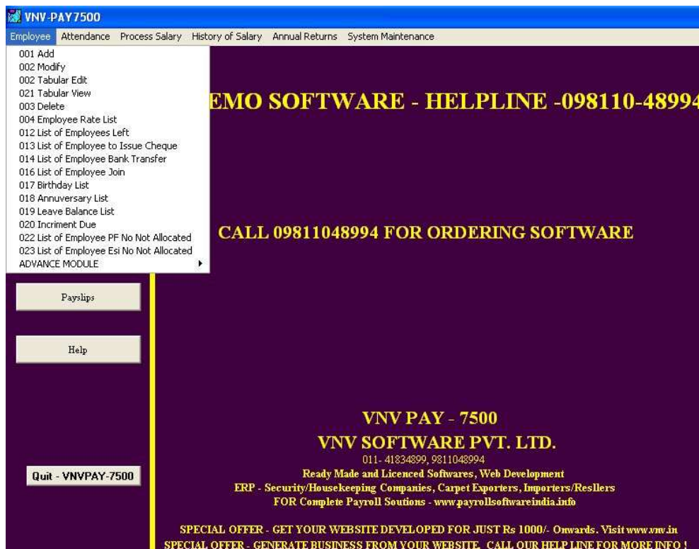
Startup screen
