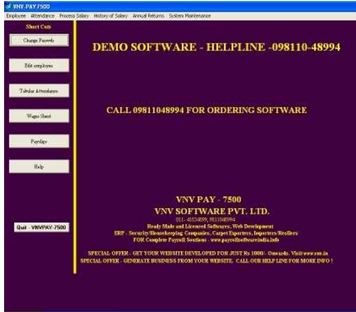
Startup screen
